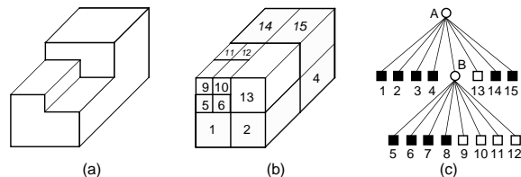
Figure 6: (a) Example three-dimensional object; (b) its octree block decomposition; and (c) its tree representation.
