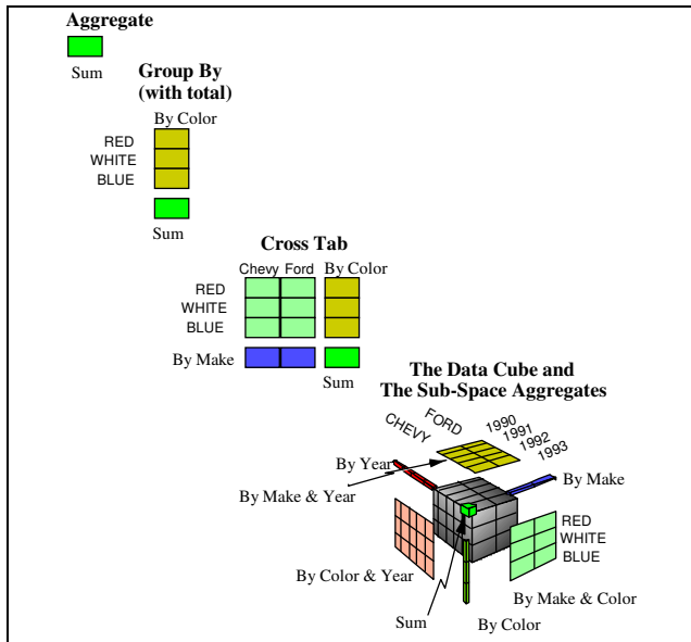
Figure 3: The CUBE operator is the N -dimensional generalization of simple aggregate functions. The 0D data cube is a point. The 1D data cube is a line with a point. The 2D data cube is a cross tabulation, a plane, two lines, and a point. The 3D data cube is a cube with three intersecting 2D cross tabs.
