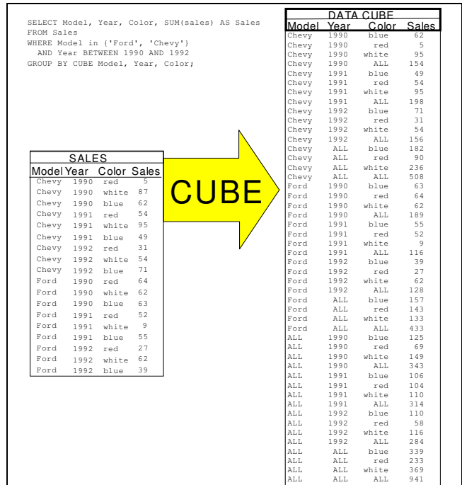
Figure 4: A 3D data cube (right) built from the table at the left by the CUBE statement at the top of the figure.
